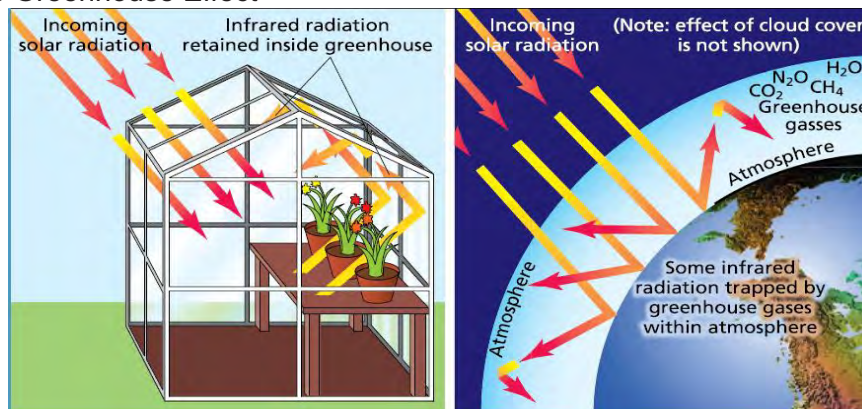
Figure 1.2: The Greenhouse Effect
