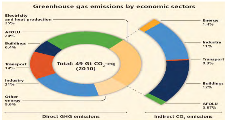
Figure 1.5: Anthropogenic greenhouse gas emissions (Gt CO 2 -eq/year) by economic sector
