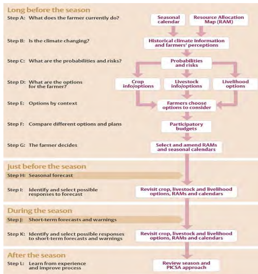
Fig 3.25 : How Climate Information Services works at different temporal scales
