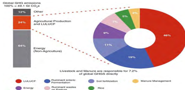
Figure 1.6: Agriculture, forestry and other land use (AFOLU) emissions by component in 2010
