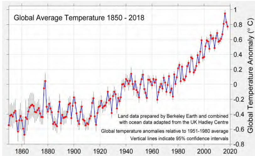
Figure 1.3: Global temperature anomaly since 1850
