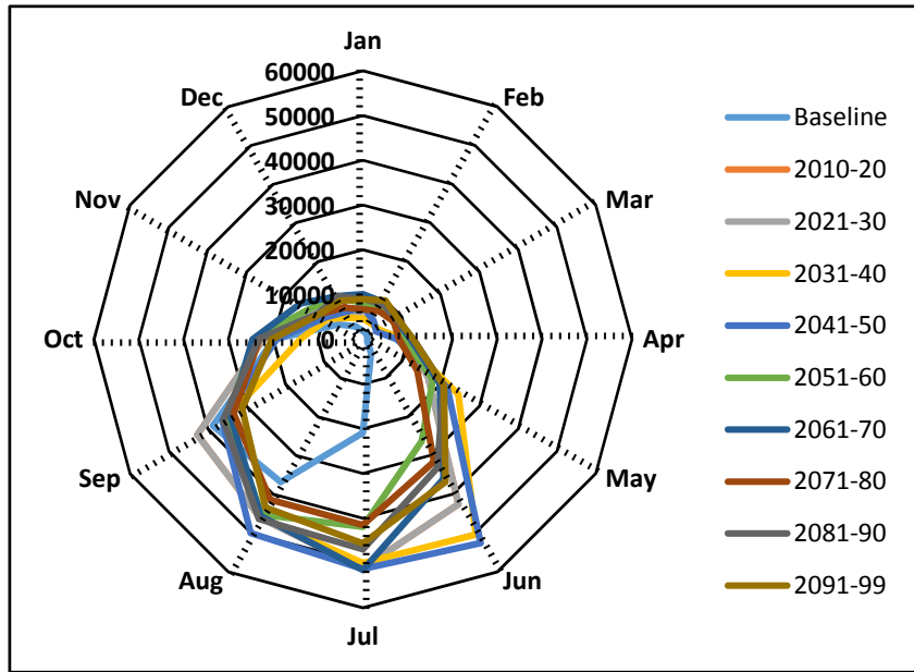
Figure 34 Average available monthly flow (m 3 /s) in the Ganges basin from the CNRM-CM5 model under RCP 4.5
