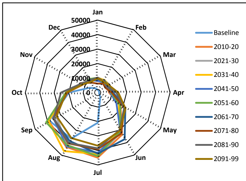
Figure 41 Average available monthly flow ( m^3/s ) in the Ganges basin from the MPI-ESM-LR model under RCP 8.5
