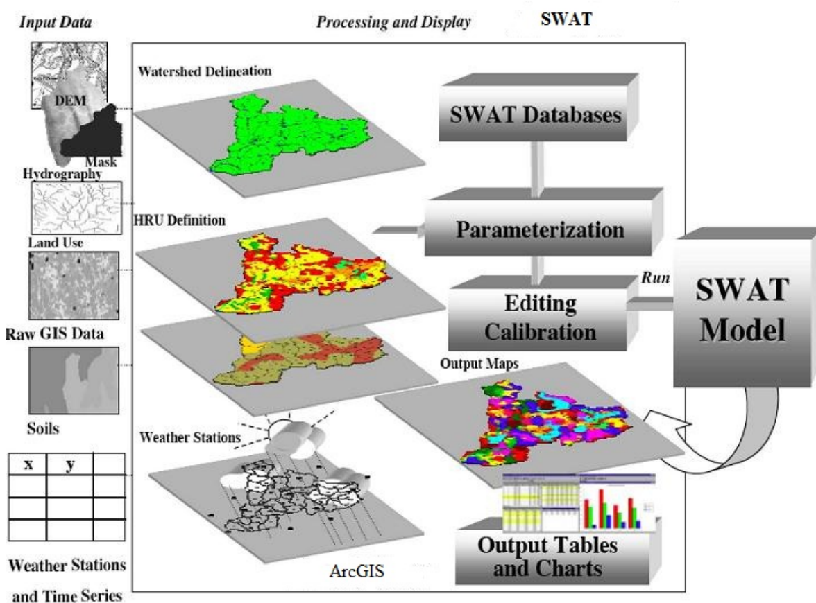
Figure 24 Schematic diagram of the SWAT model
