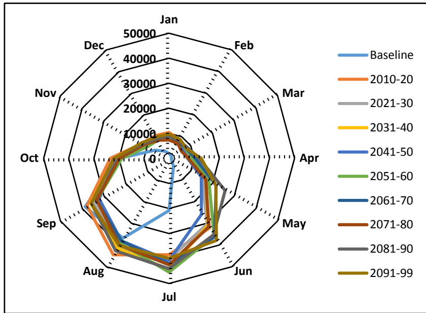
Figure 38 Average available monthly flow (m 3 /s) in the Ganges basin from the CNRM-CM5 model under RCP 8.5
