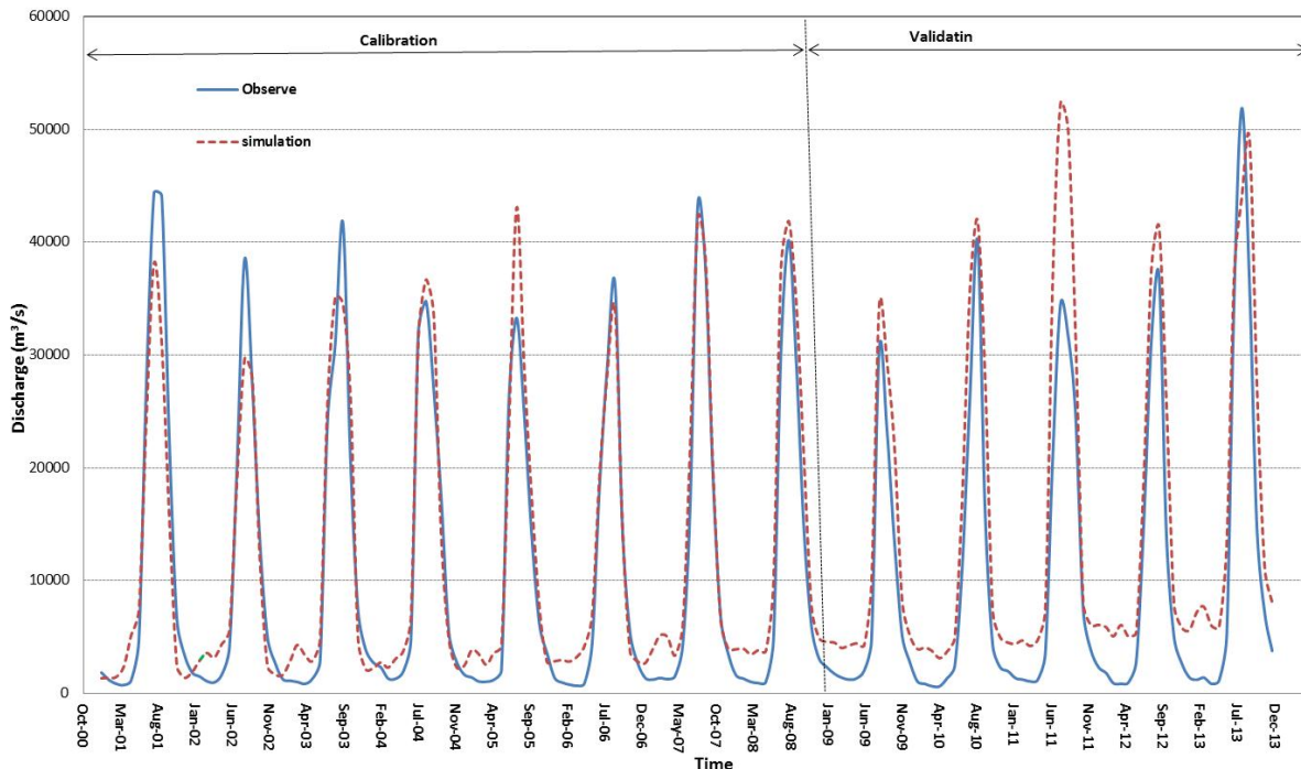
Figure 33 Calibration and validation results of the SWAT model at Hardinge Bridge, Bangladesh
