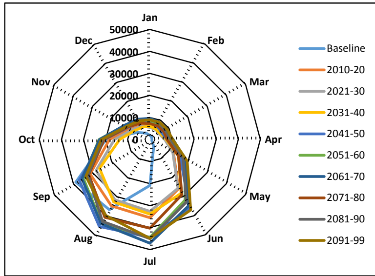
Figure 42 Average available monthly flow (m³/s) in the Ganges basin under RCP 4.5 (an ensemble of four GCMs)
