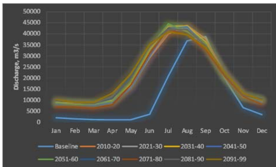
Figure 45 Monthly variation of the available flow in the Ganges basin under RCP 8.5.
