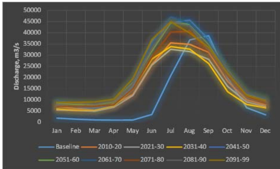
Figure 44 Monthly variation of the available flow in the Ganges basin under RCP 4.5
