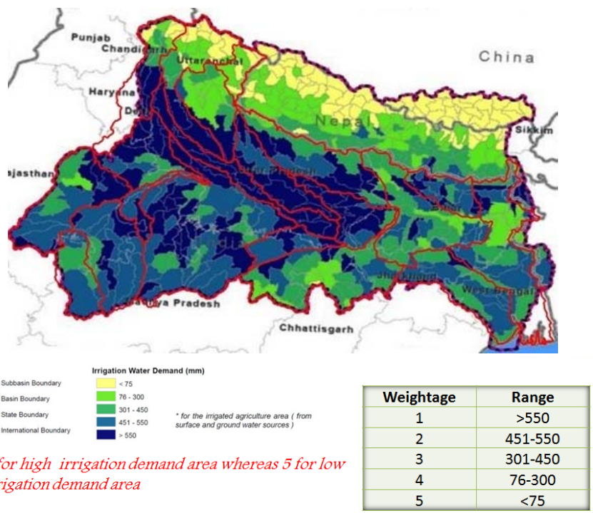
Figure 7 Irrigation water demand in the Ganges basin
