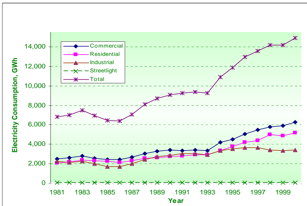
Figure 4-4-7-6: 1981 to 2000 CO 2 emissions from electricity consumption, by consumer type in Metro Manila
