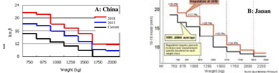
Figure 4-4-3-9 Fuel economy level of new cars
