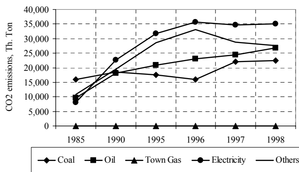
Fig.4-4-2-7: CO 2 emissions of Shanghai by fuel type
