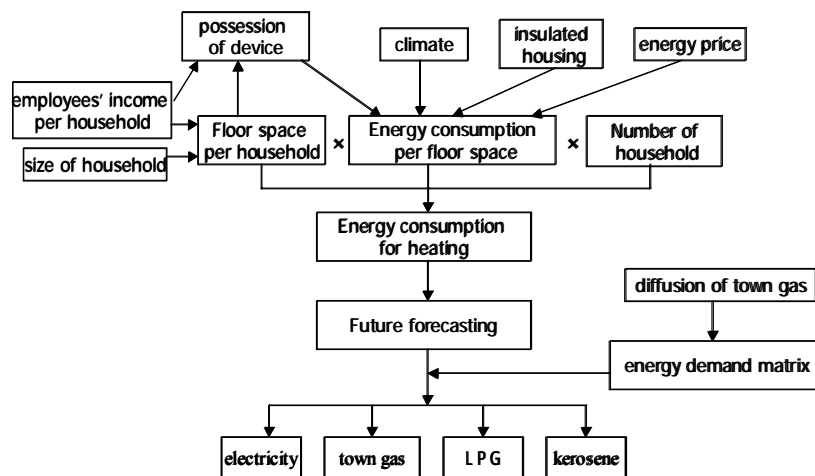
Figure 4-4-10 Estimation of energy consumption for heating
