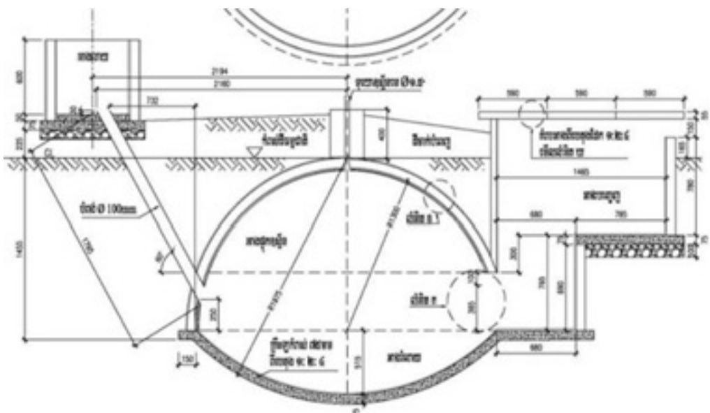
Figure III-2 Farmer's Friendly Biodigester Plant modified by NBP
