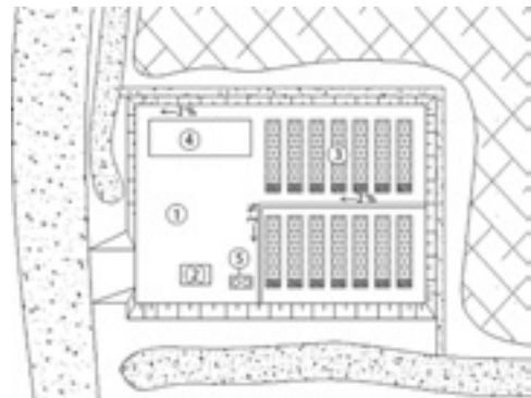
Figure II.1 Sketch map of COMPED Composting plant at Stung Meanchey
